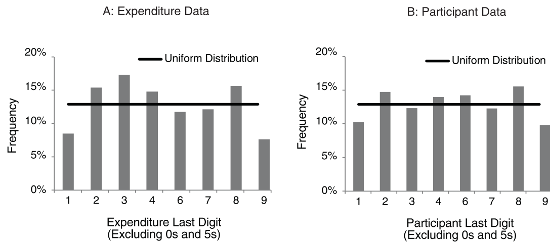
Figure 11. Last-digit expenditure and participant data against the uniform distribution.
