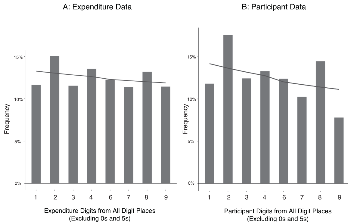
Figure 2. All digit places beyond the first vs Benford's Law for expenditure and participant data.
