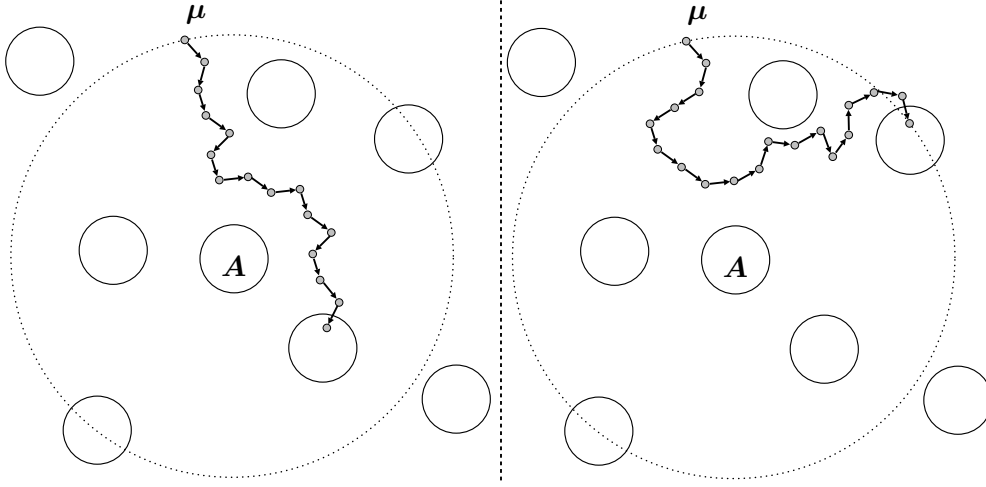
Figure 1: Theorem 1, blocking paths that do not “wander off”
