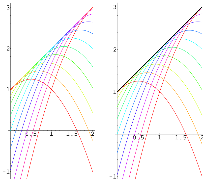
Figure 3. Graph of V(p) = p + 1 as the envelope of the family of curves \{\varphi_x(p) : x = 0.0, 0.2, \dots, 2.0\} , where \varphi_x(p) = p - (x - p)^2 + 1 = f(x, p) .
